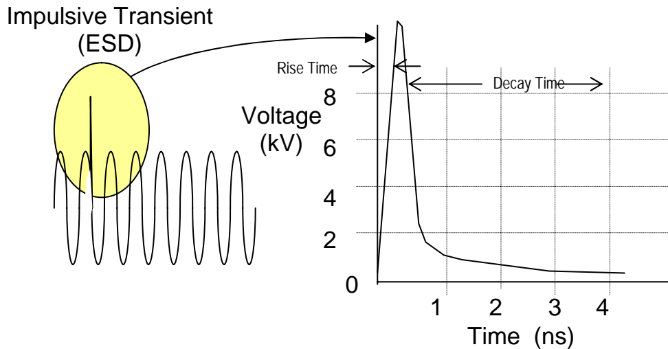
Figure 2 – Positive impulsive transient
