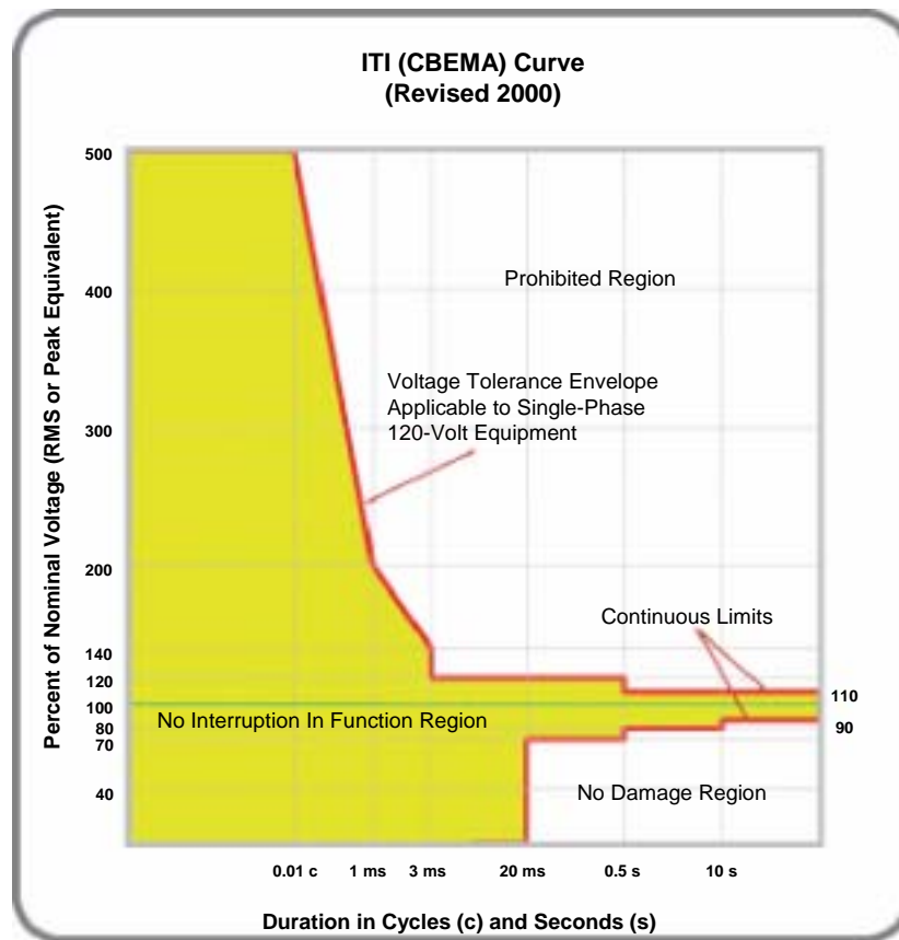
Figure A1 – ITIC curve
