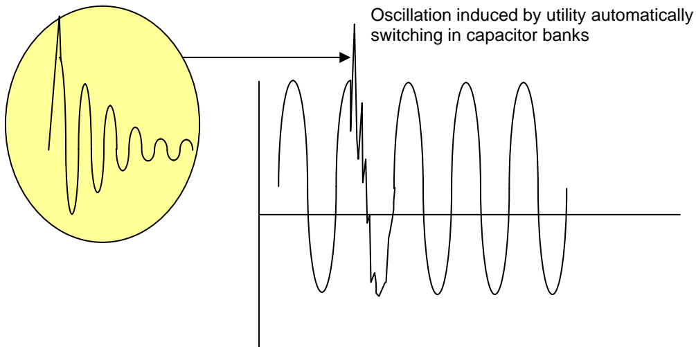
Figure 4 – Oscillatory transient
